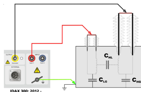
Fig. 7: Example of connections to a two-winding transformer All IDAX have 3 measurement terminals (red, blue and ground) that allows measuring multiple tests in an automatic sequence without having to change cable connections on the transformer.
